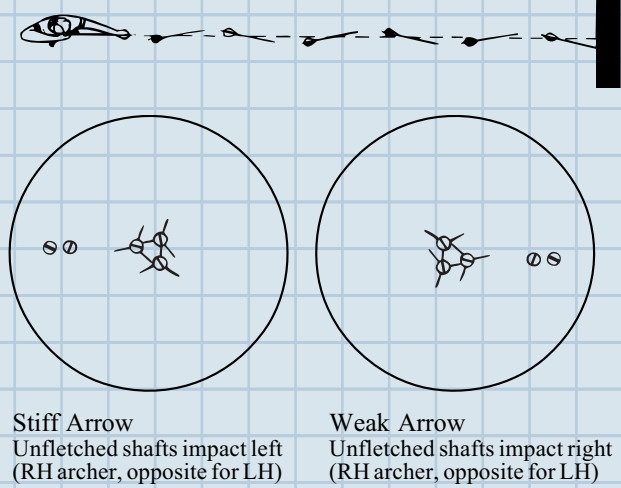
Fig. 11 Fishtailing
