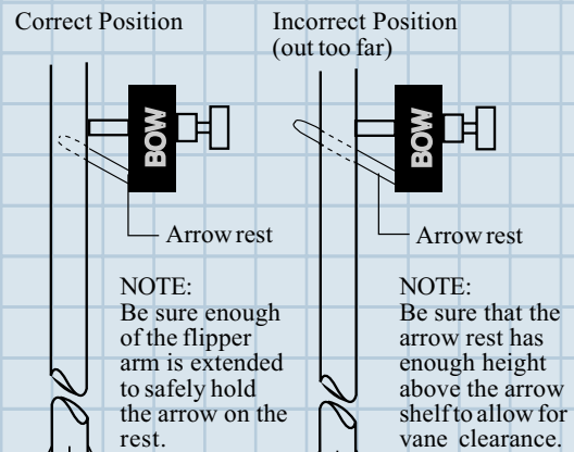
Arrow Rest - Overhead View (RF, CF)
