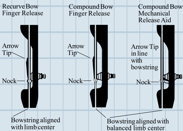
Fig. 7 - Arrow Centering
