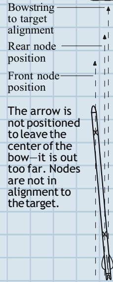
Fig. 6 Misaligned Arrow RF, CF, CR (Incorrect Arrow Rest Position)
